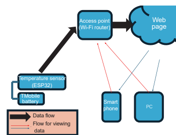
System for collecting measurement data
