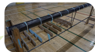
Making prototype of wing part on workbench built from scrap wood
